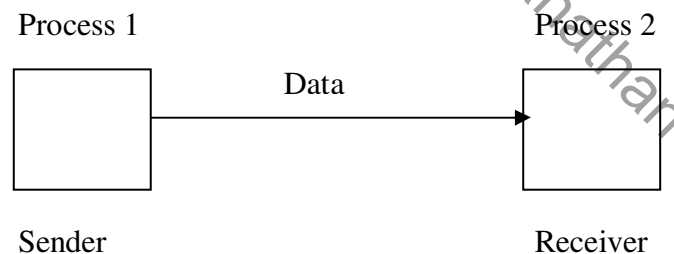
Figure 1: Interprocess Communication
