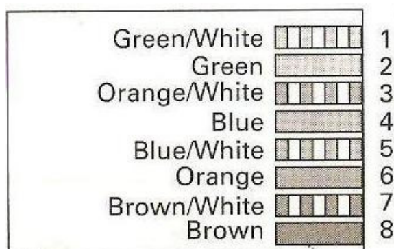
Figure 20: TIA/EIA 568A Standard
