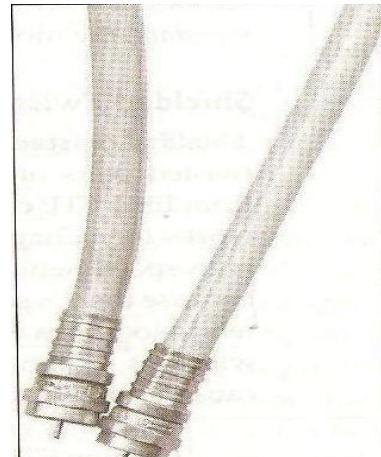
Figure 4: RG-62 cable
