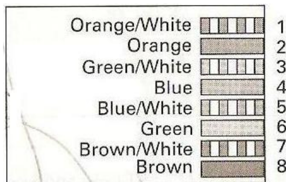
Figure 21: TIA/EIA 568B Standard
